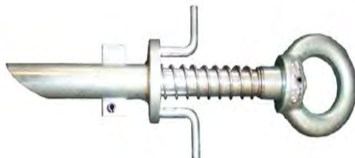
Model 00650 – Grip Anchor Fits 11/16" to 1" diameter holes Maximum depth - 1-9/16" Can be used horizontally or vertically 5,000lb Anchorage Point
